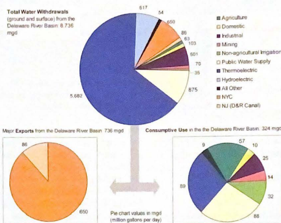
Fig 1.10. Daily Water Withdrawals, Exports and Consumptive Use in the Delaware River Basin
