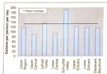
Fig. 1.8. Regional Per Capita Water Use.
